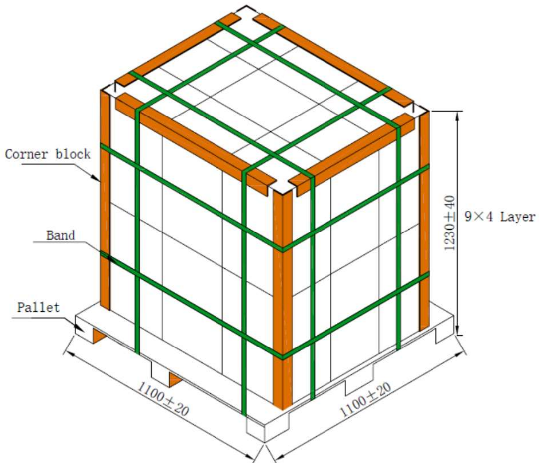
Fig. 4. Air transportation package
